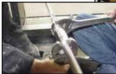
Design-Build Retrofit Assembly of curtainwall cable system and finished installation
